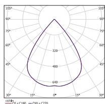
Le curve fotometriche si riferiscono ai 2 LED naturali e sono indicative Photometric curves refer to the 2 LEDs Natural White and are indicative
