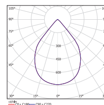
Le curve fotometriche si riferiscono ai 6 LED naturali e sono indicative Photometric curves refer to the 6 LEDs Natural White and are indicative
